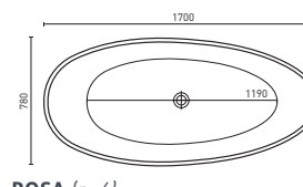
ROSA (p. 6) 1700 x 780 x 655 mm (177L)
