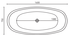
SHERATON (p. 8) 1600 x 750 x 595 mm (125L)
