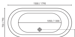
COOL (p. 7) 1500 x 750 x 580 mm (140L) 1790 x 790 x 580 mm (155L)
