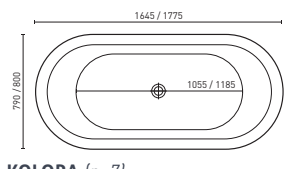
KOLORA (p. 7) 1645 x 790 x 580 mm (144L) 1775 x 800 x 580 mm (155L)
